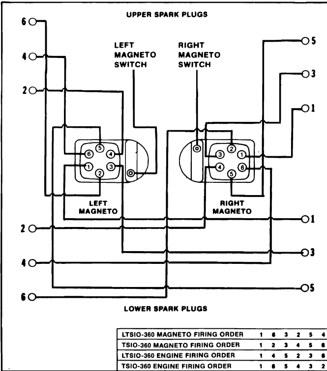
FIGURE 71 IGNITION WIRING DIAGRAM
