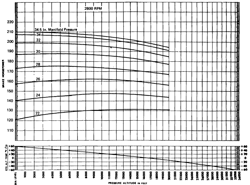
FIGURE 30 ALTITUDE PERFORMANCE AT 2800 RPM TSIO-360-H, HB
