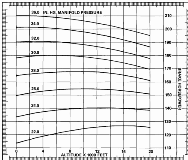
FIGURE 41 ALTITUDE PERFORMANCE AT 2700 RPM TSIO-360-JB
