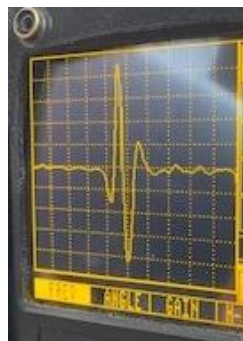
Eddy Current Indication of 0.030" x 0.030" reference Notch for Calibration
